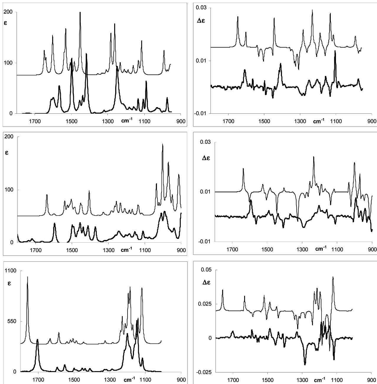
Figure 3. Comparison of experimental (bold trace) and calculated (lighter trace) IR (left) and VCD (right) spectra for 4-X-[2.2]paracyclophanes (X = F (1), top, X = CH 2 F (2), middle, X = COCF 3 (3), bottom) in the mid-IR region. (See text.) Only the ( R )-enantiomer reported. For X = CH 2 F the average calculated spectra according to \Delta G are reported.
